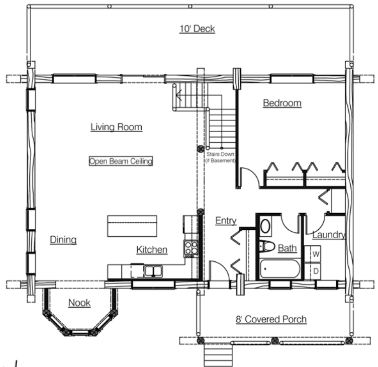
Main Floor
