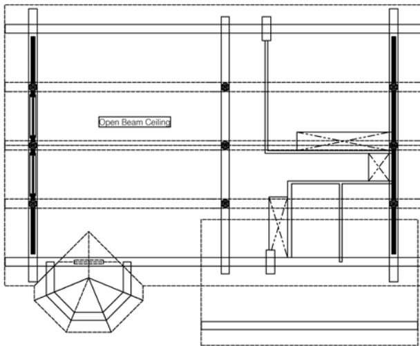
Roof Plan
