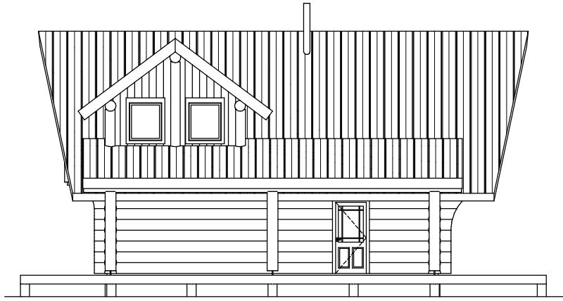
Left Elevation
