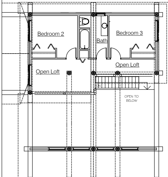
Loft Floor
