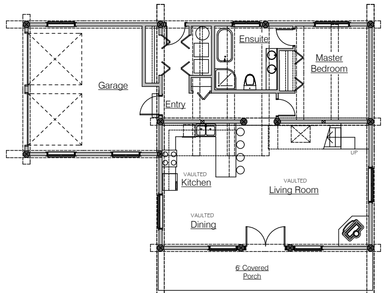
Main Floor
