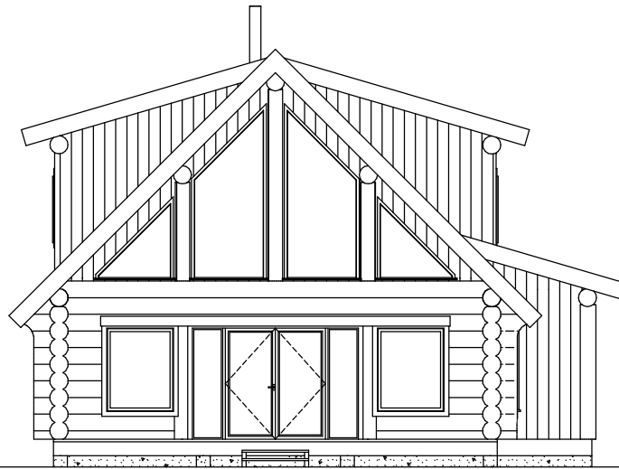
Front Elevation
