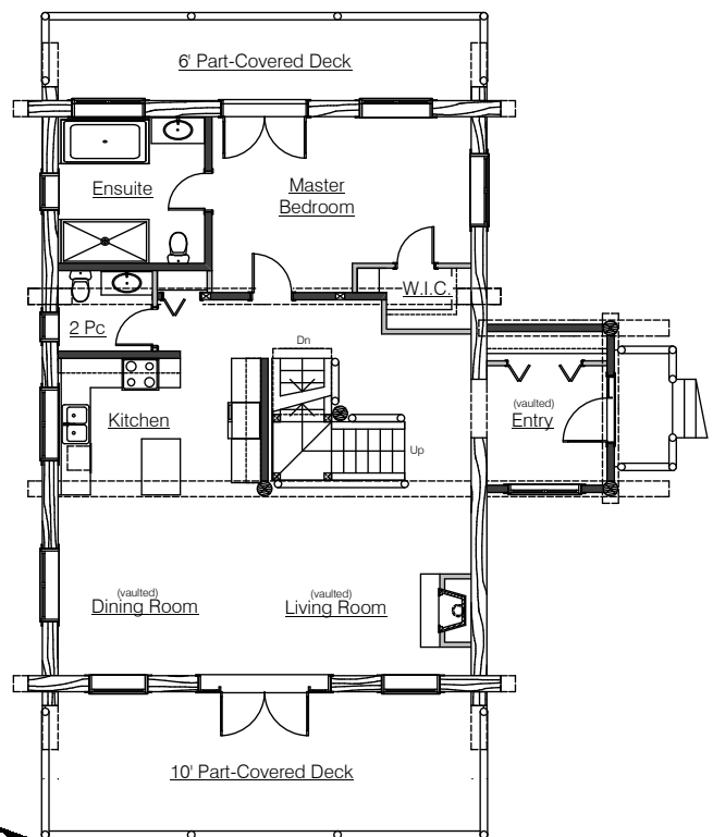
Main Floor
