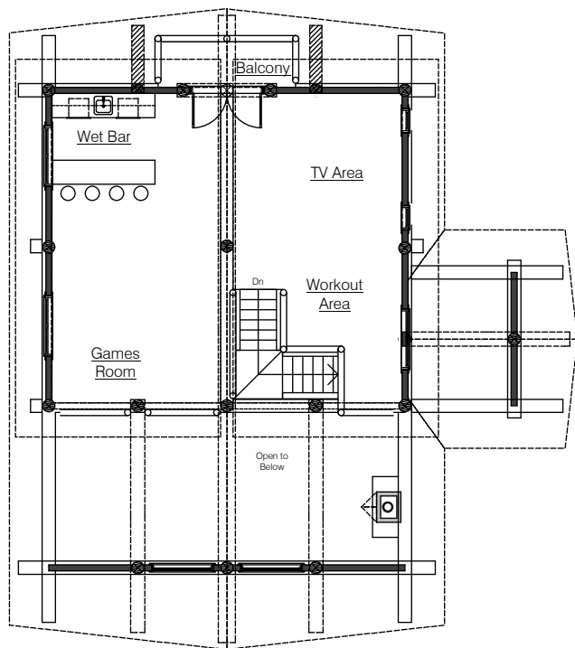
Loft/Roof Plan
