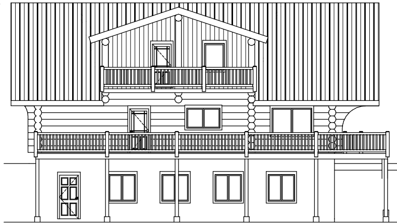
Left Elevation
