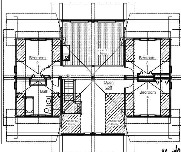
Loft/Roof Plan
