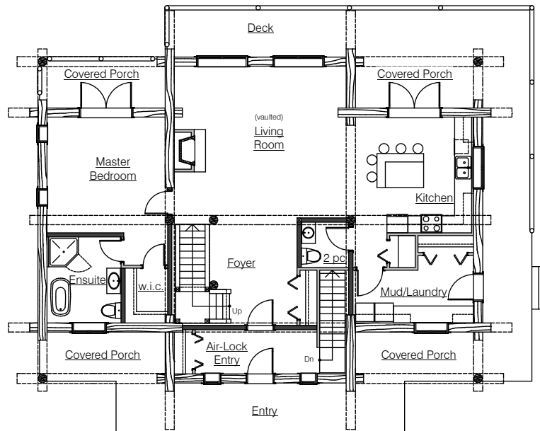
Main Floor
